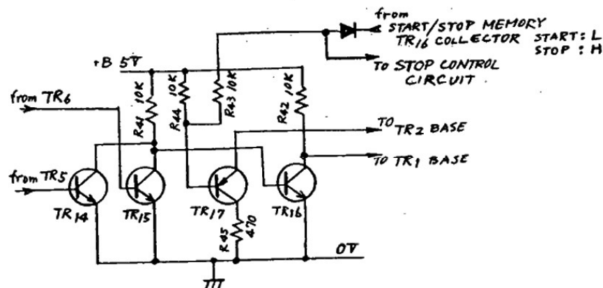
DIAGRAM 9 MIXING CIRCUIT
