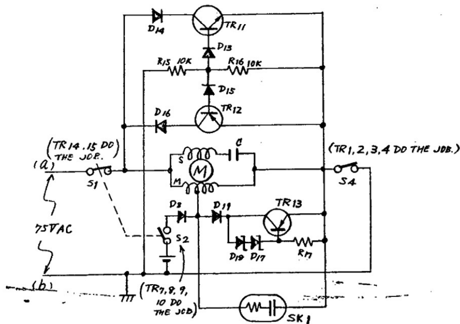
DIAGRAM 14 SPIKE SNUBBERS
