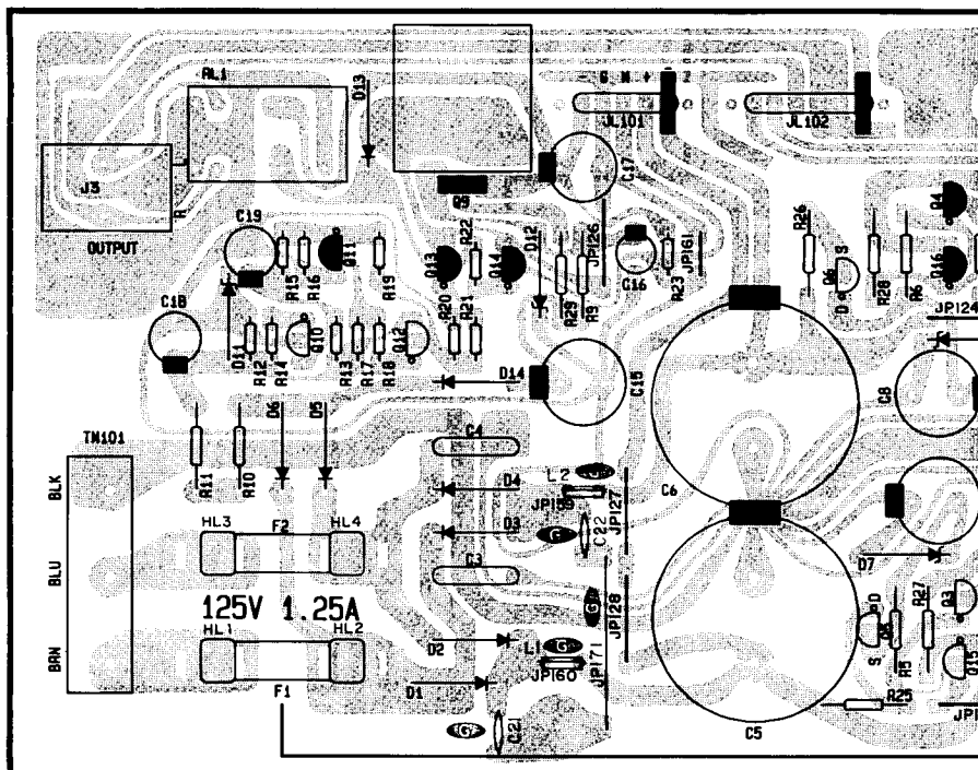
PCB-1 Power Supply P. C. Board
