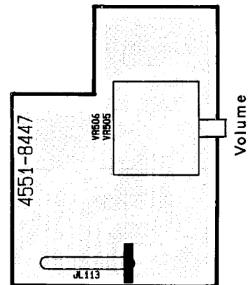
PCB-5 Volume P. C. Board
