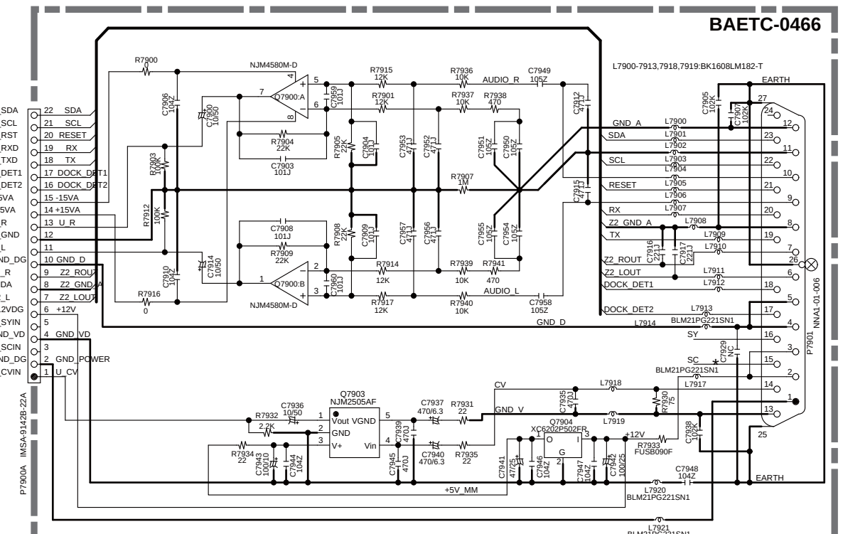
U0054 UNIVERSAL PORT PC BOARD BAETC-0466
