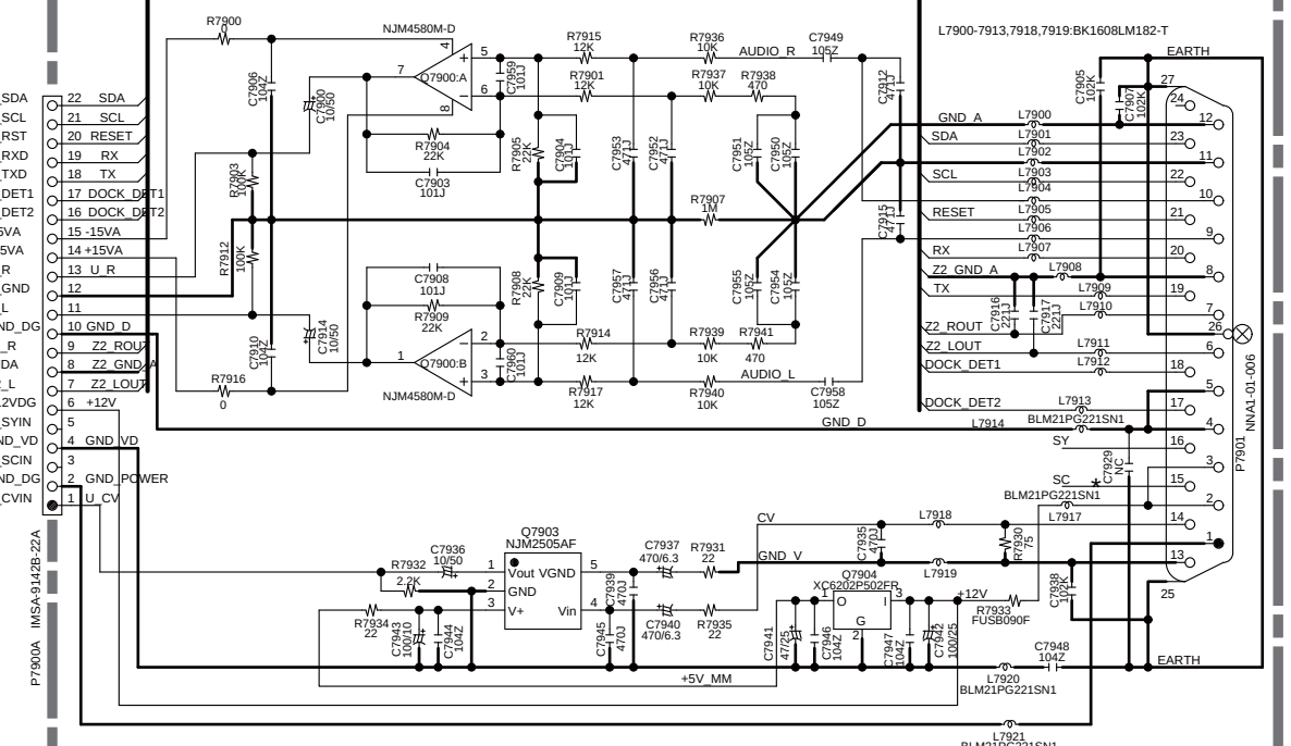
U0054 UNIVERSAL PORT PC BOARD BAETC-0466
