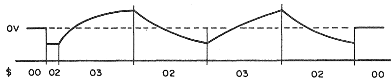
Fig. 4-7. Search Voltage Creation by $02 and $03 (Pin 11 Voltage)
