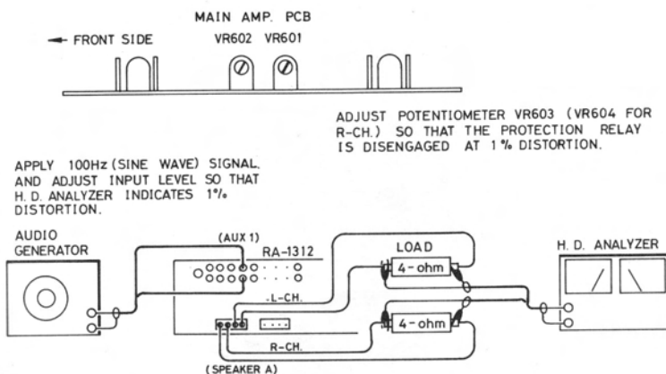
Fig.3 OVERLOAD PROTECTION LEVEL ADJUSTMENT HOOK-UP
