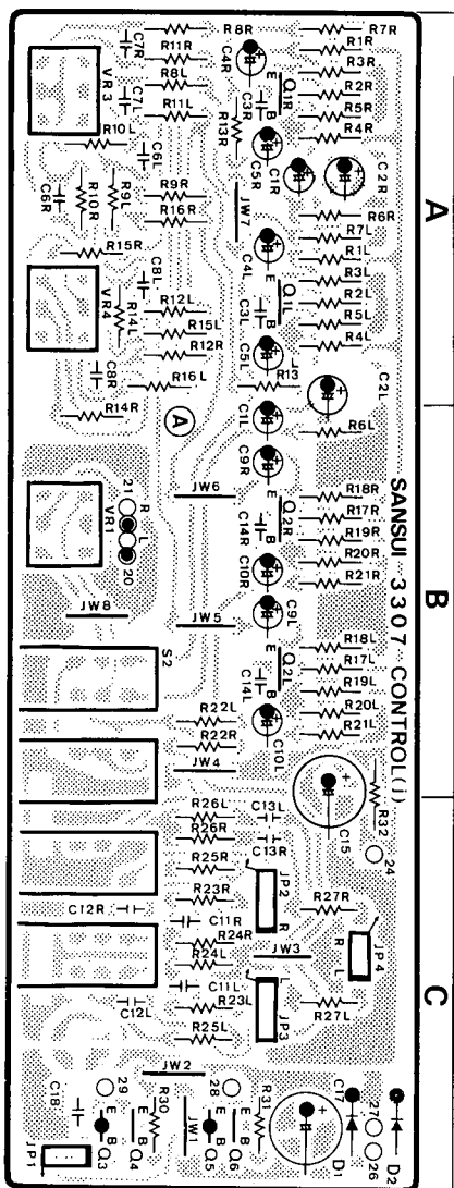
5-7. F-3307 Tone Control Circuit Board (Stock No. 00613301 = 9900Z, 8900ZDB)
