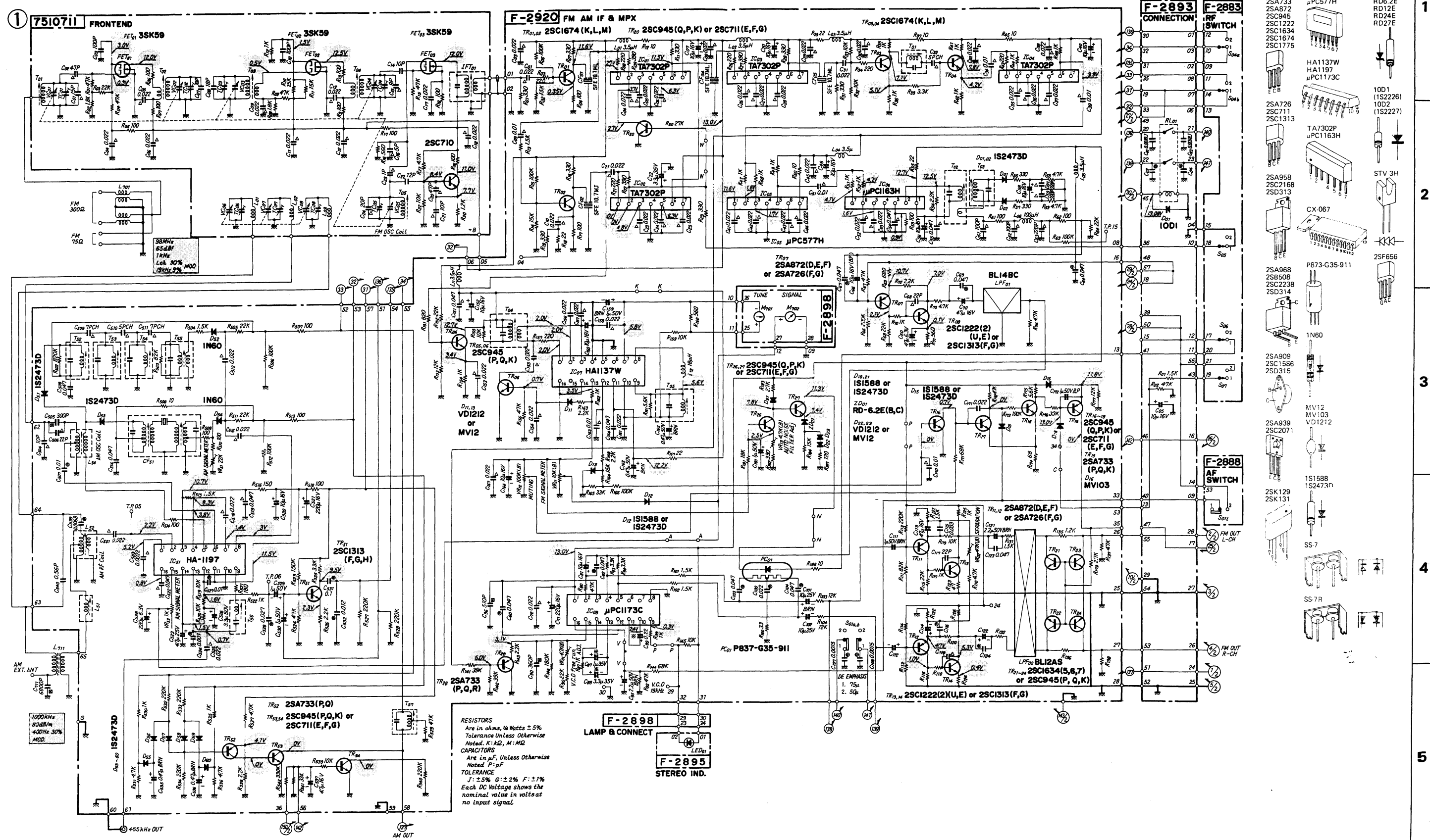
8-1. Tuner Section <G-22000/G-33000>
