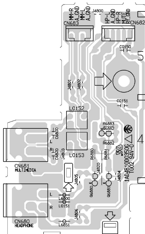
HEADPHONE P.W.BOARD
