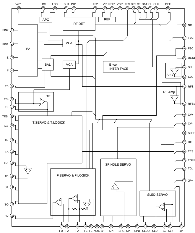
LA9240M (Servo Signal Processor)
