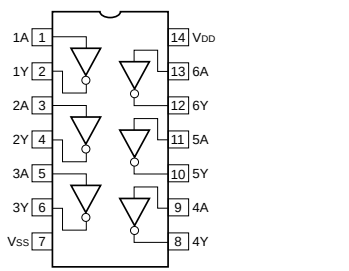
IC608 : TC74HC044P Hex Inverters
