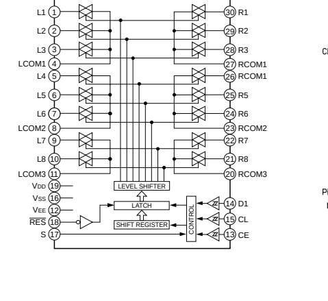
IC505, 522 : LC78213 Analog Function Switch
