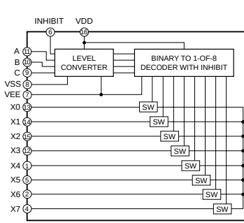
IC602-605 : TC74HC4051AP Analog Multiplexer/Demultiplexer
