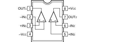
IC501 : NJM2068MD-T1 IC506-508, 511, 513-515, 521, 523-525 : uPC4570G2 Dual OP-Amp
