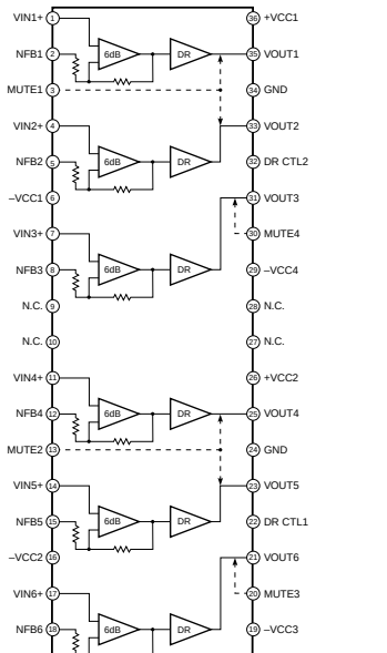
IC609 : LA7109 75Ω Video Driver
