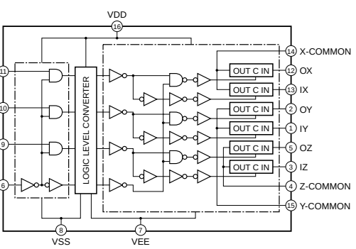
IC607 : TC74HC4053AP Triple 2-Channel Multiplexer/Demultiplexer
