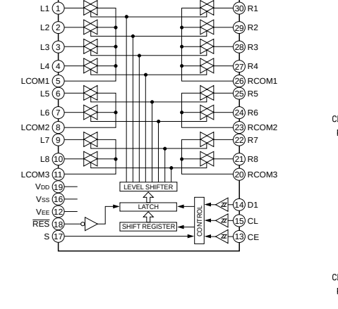
IC505, 504 : LC78212 Analog Function Switch
