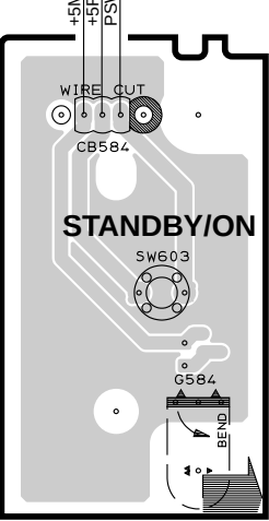
FUNCTION (5) P.C.B. (Lead Type Device)
