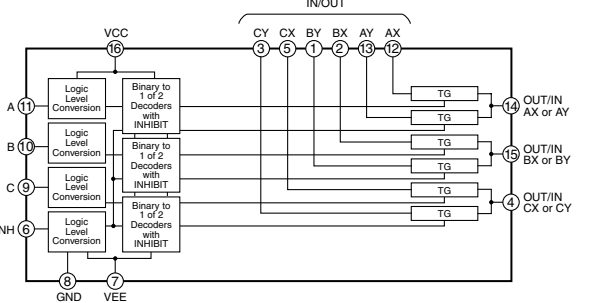
IC327: MM74HC4053SJX Triple 2-channel analog m
