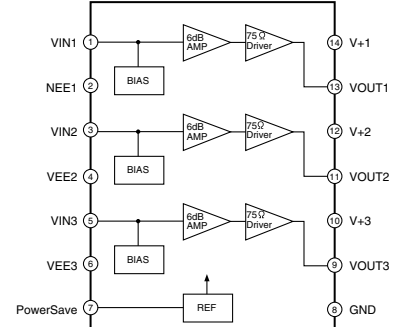
IC325: NJM2581M Video amplifier
