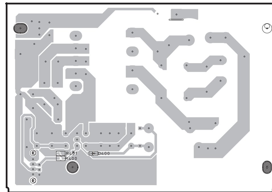
SUB (2) P. C. B. (Surface Mount Device)
