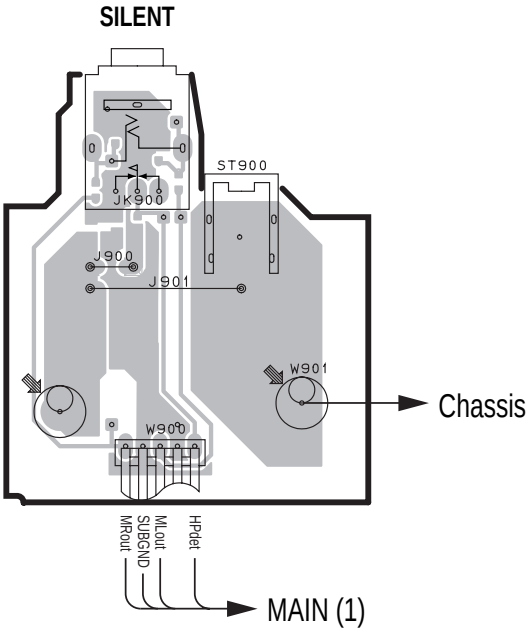
SUB (5) P. C. B. (Lead Type Device)
