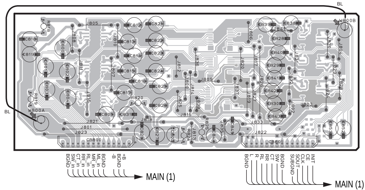
SUB (1) P. C. B. (Surface Mount Device)
