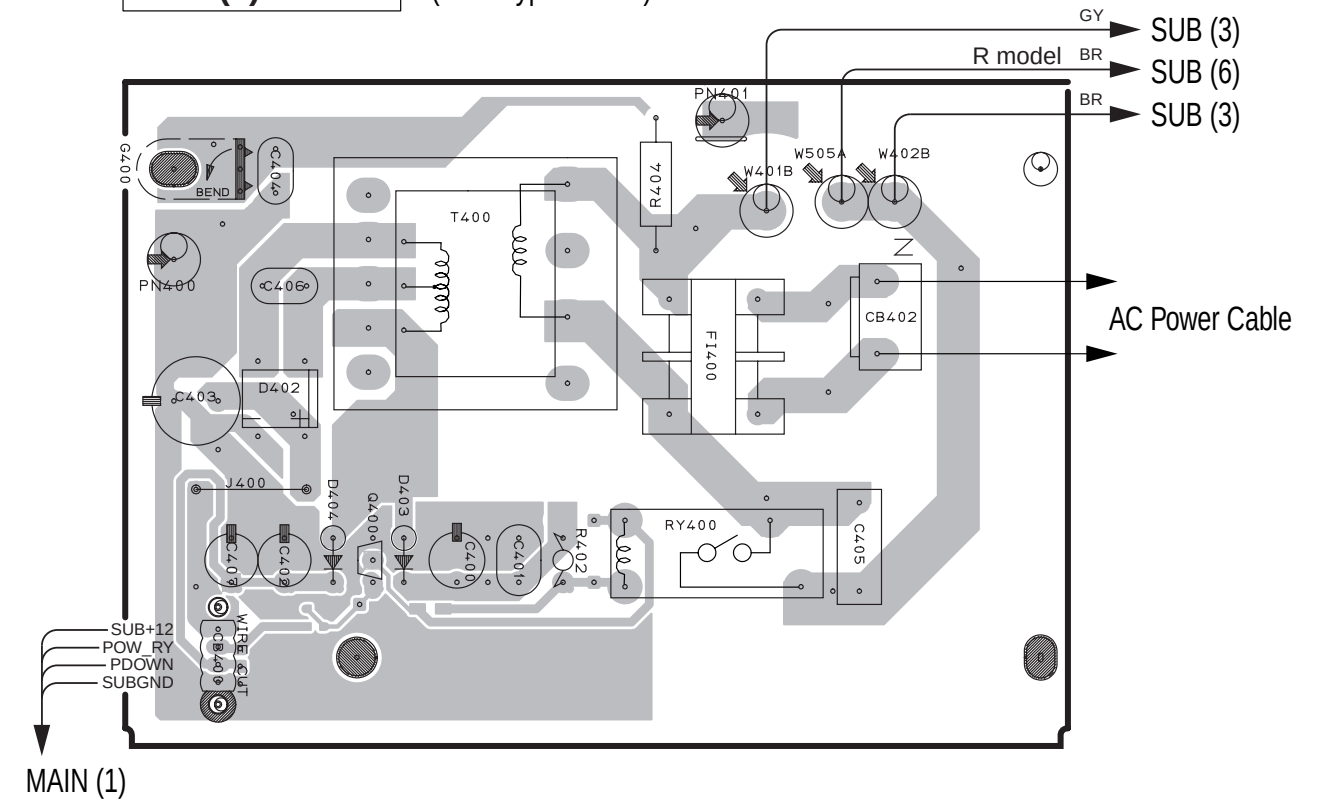
SUB (2) P. C. B. (Lead Type Device)
