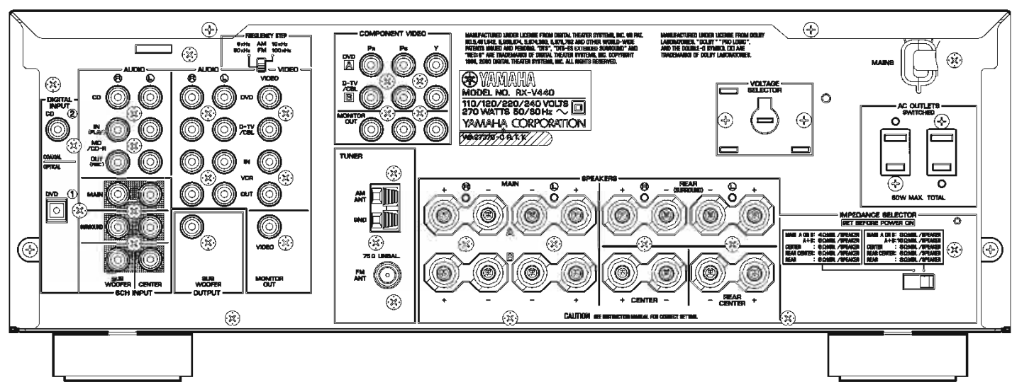
RX-V440 (R model)
