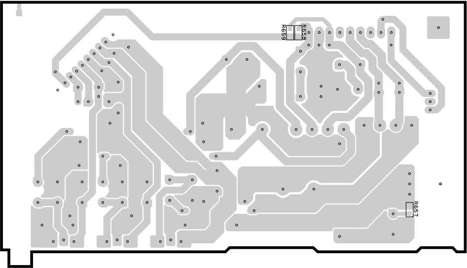
FUNCTION (4) P.C.B. (Surface Mount Device)
