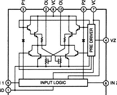
IC404 : LB1641 Motor Driver
