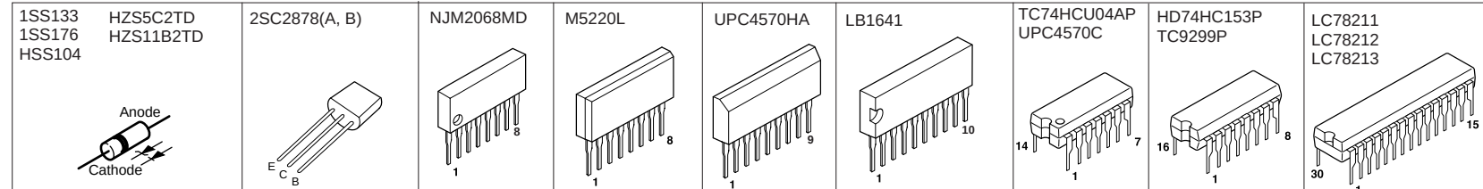
PIN CONNECTION DIAGRAM OF DIODES, TRANSISTORS AND IC'S.
