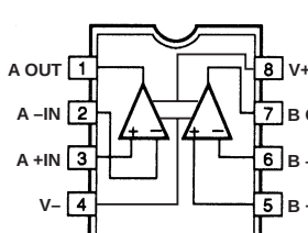
IC401-403 : \mu PC4570C Dual OP-Amp
