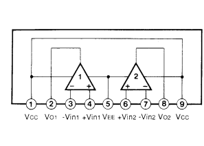
IC105, 106, 112, 113 : \mu PC4570HA Dual OP-Amp
