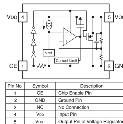
IC45: R1172H121D-T1-F CMOS-based positive-voltage regulator IC
