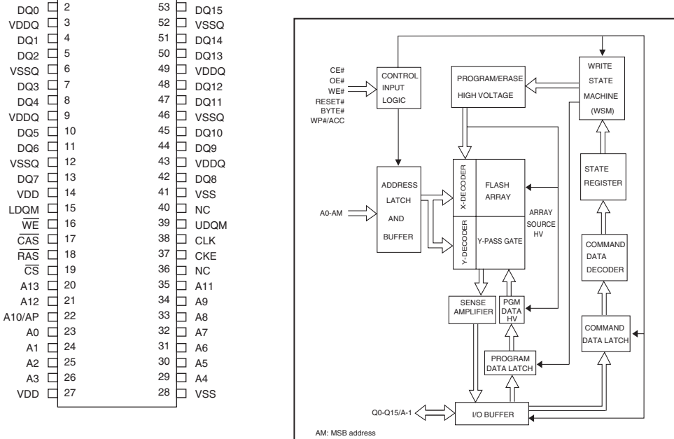
IC43: MX29LV160DBT1-70G 16 M-bit 3 V supply flash memory
