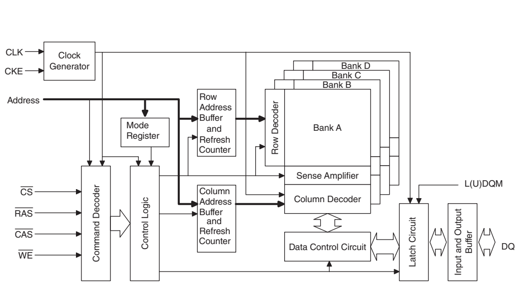
IC42: M12L64164A-STG 1M x 16-bit x 4 banks synchronous DRAM
