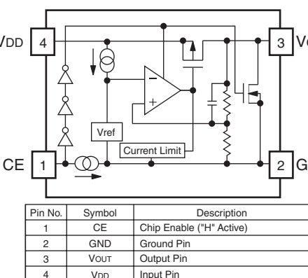
IC44: RP130Q501D-TR-F Voltage regulator
