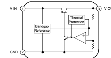
IC22: NJM2845DL1-18 Low dropout voltage regulator
