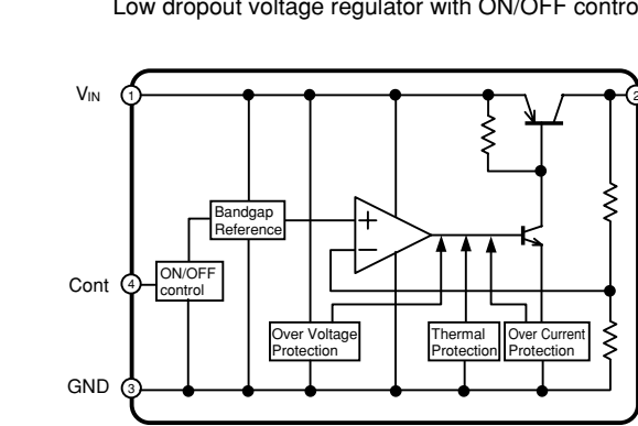
IC707: NJM238F63 Low dropout voltage regulator with ON/OFF control
