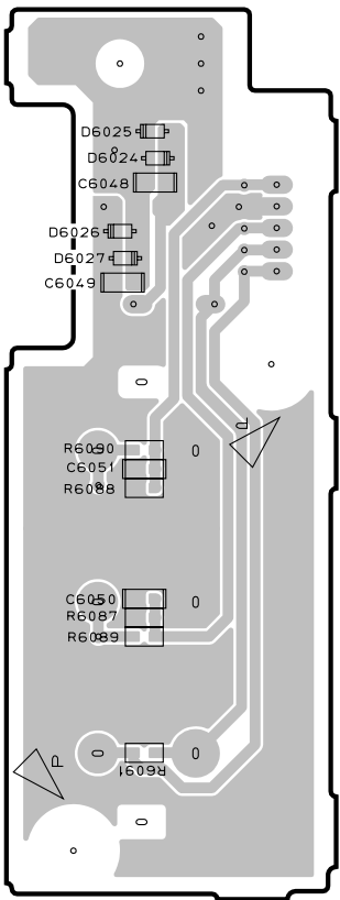
OPERATION (4) P.C.B. (Side B)
