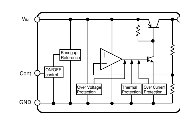
IC706: NJM238F05 Low dropout voltage regulator with ON/OFF control
